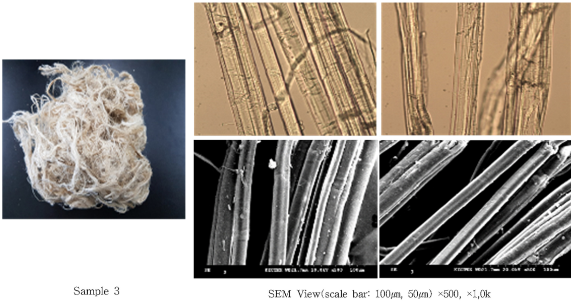
Fig. 7. SEM image of sample 3 after degumming.
