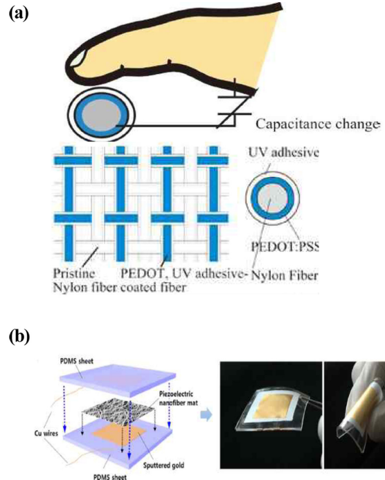
Fig. 3. Pressure and force sensors. (Park et al., 2016; Takamatsu et al., 2011).
