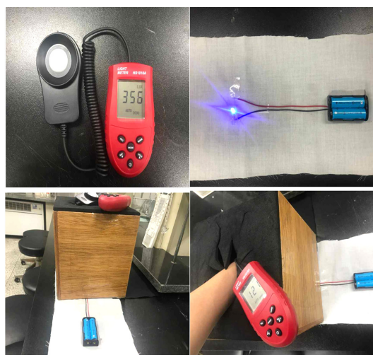
Fig. 5. Measuring of LED lamp consistency(lux).
