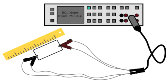
Fig. 4. Schematic of measuring electrical resistance.
