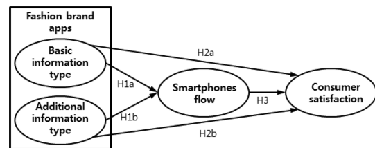
Fig. 1. Research model.
