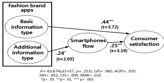
Fig. 2. Structural model.
