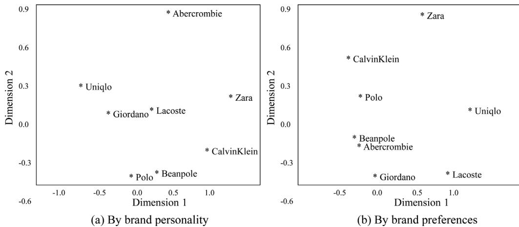
Fig. 1. Multi-dimensional scaling analyses.
